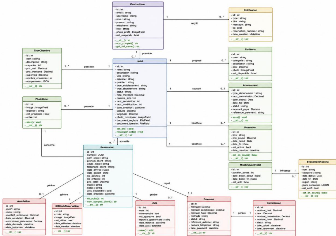
Figure 14: Diagramme de classes
